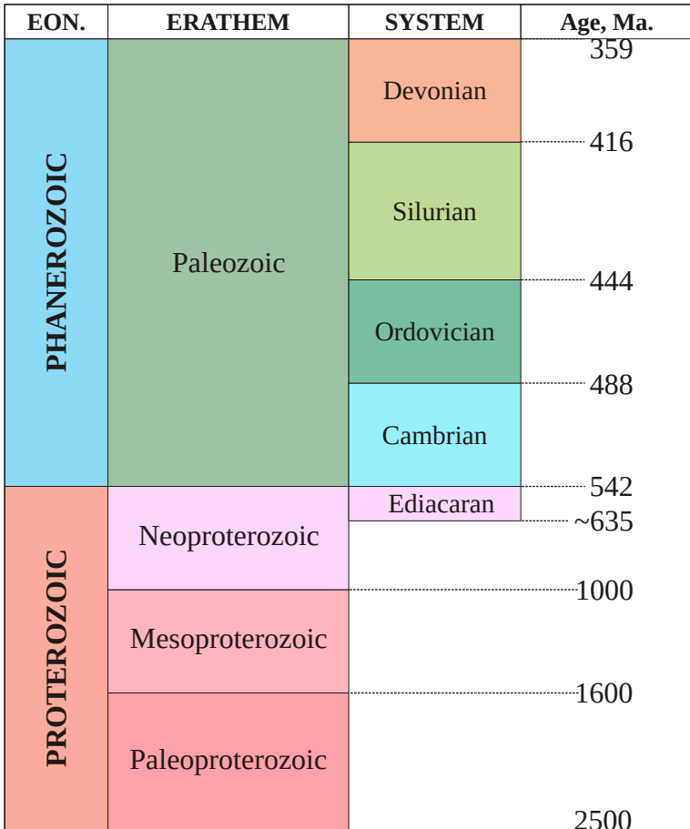
Stratigraphic scheme of the Estonian bedrock. Ages correspond to the ICS International Stratigraphic Chart (2009).
